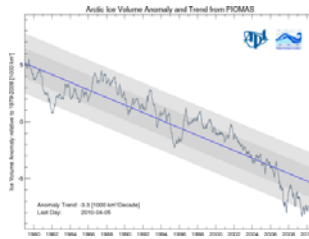
APL-UW PSC, J. Zhang (2010)
