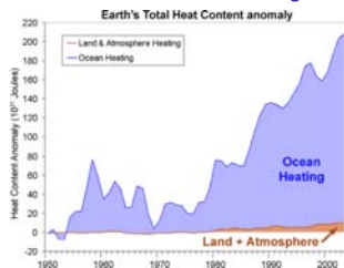
Total Earth Heat Content from 1950 (Murphy 2009). Ocean data taken from Domingues et al 2008
