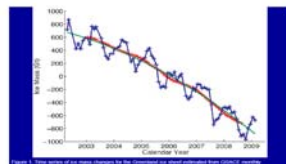
I. Velicogna, Geophysical Research Letters, 2009
