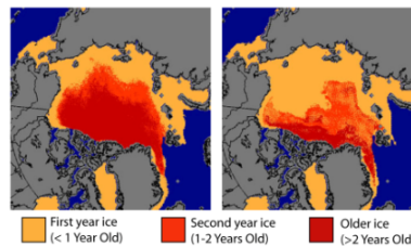
APL-UW PSC, J. Zhang (2010)
